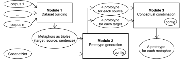
Figure 1: The pipeline architecture of \mathbf{MET}^{\text{CL}} .
